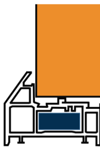
Low UPVC Usually 50-60mm
